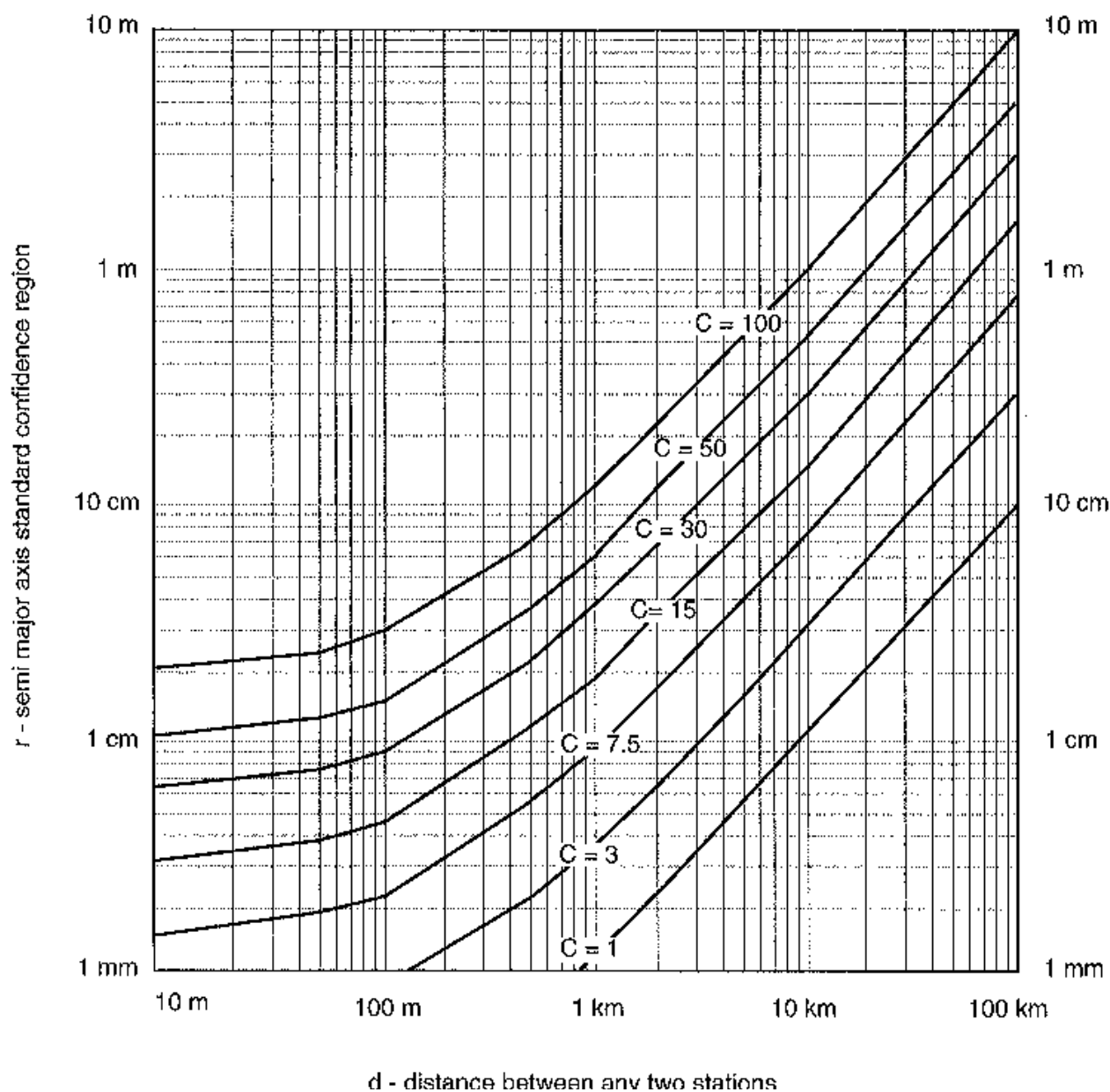
Figure 1 Horizontal Control, 2-dimensional Surveys, CLASS related values
